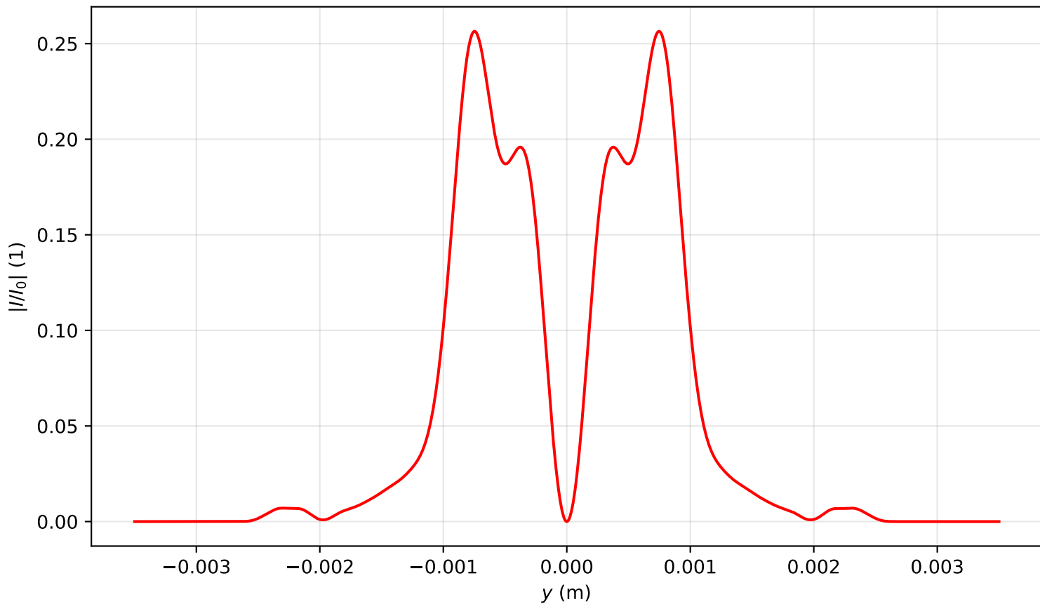
Intensity profile I(x=0, y, z=2.229)/I_0 , P_{in}=5.0P_{cr} , artificial time
